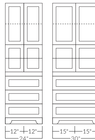
4 DOOR/3 DRAWER MODELS
