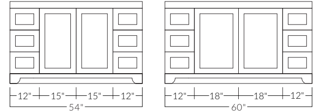
2 DOOR/6 DRAWER MODELS
